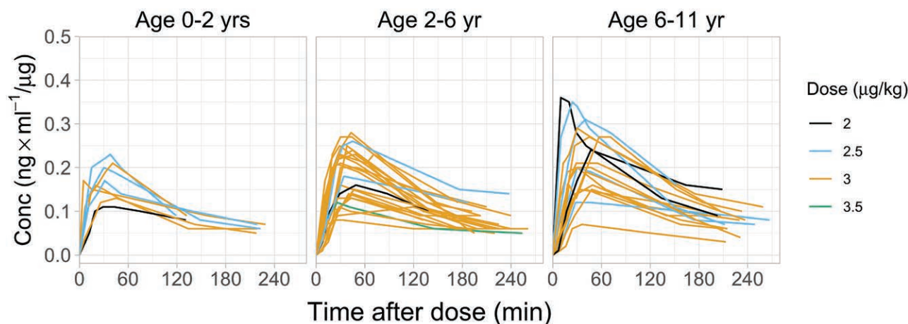
Figure 1. Dose-corrected dexmedetomidine concentrations in plasma after intranasal 2\text{--}3 \mu\text{g}\cdot\text{kg}^{-1} dexmedetomidine dose as nasal spray in 50 ambulatory pediatric patients in the 3 age groups (0- to 2-y olds, 2- to 6-y olds, and 6- 11-y olds). Individual doses were rounded to the nearest 10 \mu\text{g} and shown as different dosing schemes highlighted with colors. Conc indicates concentration of dexmedetomidine in plasma.
